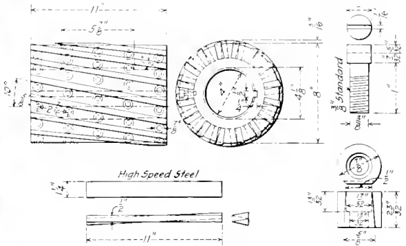
Fig. 8—Milling Cutter for Slab Milling
